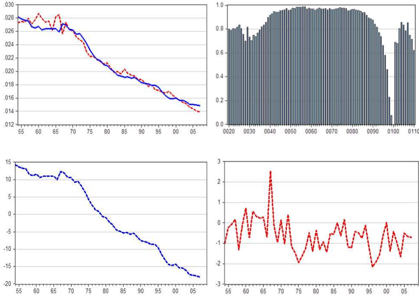
Figure 1: Lee-Carter Fitted mortality and pseudo out-of-sample (1991-2007) projections. Figure 1.1: Fitted mortality rates at 65. Figure 1.2: Cross-Sectional R^2 of Equation (3) Figure 1.3: The unobservable mortality index k_t . Figure 1.4: Innovations in k_t .
