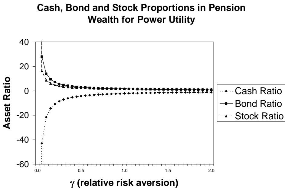
Fig.2 The relationship between \gamma and the optimal proportions of cash, bond and stock invested for v_{rS} = 1 . The \gamma range is cut off at 2 in order to show the full extent of cash short-sale and purchase of bond and stock.
