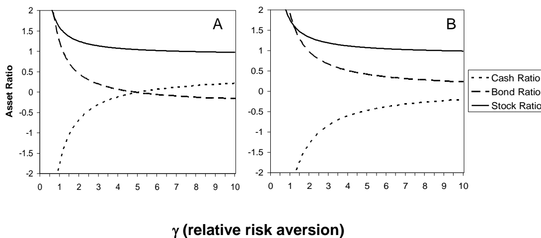
Fig. 1 The relationship between relative risk aversion coefficient \gamma and the optimal proportions of cash, bond and stock invested for pension wealth. The asset ratio range is cut off at -2 and 2 in order to show details of asset proportion when \gamma > 1 . A. Interest volatility scale factor for stock, v_{rS} = -1 . B. v_{rS} = 1 .
