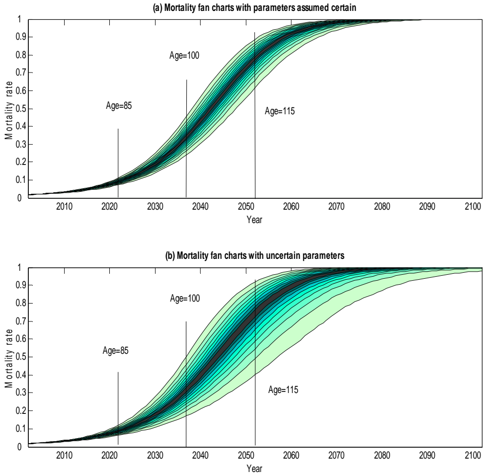
FIGURE 1: MORTALITY FAN CHART FOR COHORTS OF MALES CURRENTLY AGED 65 YEARS OLD
