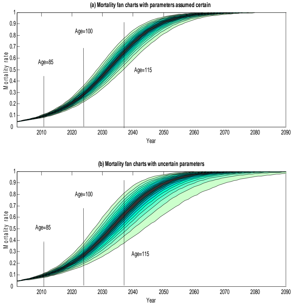
FIGURE 2: MORTALITY FAN CHART FOR COHORTS OF MALES CURRENTLY AGED 75 YEARS OLD
