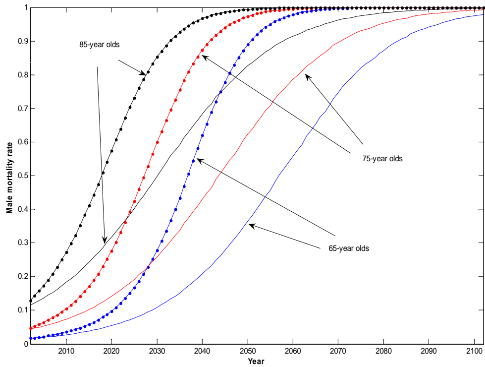
FIGURE 4: 90% PREDICTION BOUNDS FOR MALE MORTALITY RATES
