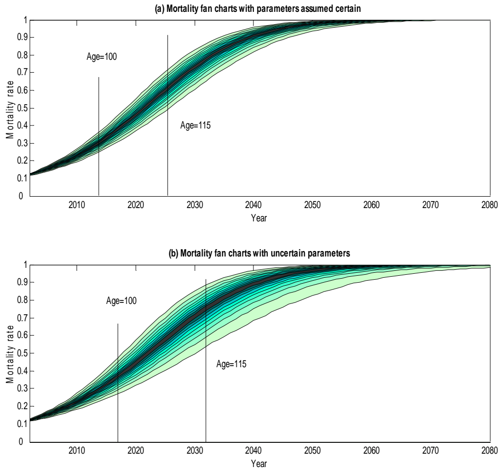
FIGURE 3: MORTALITY FAN CHART FOR COHORTS OF MALES CURRENTLY AGED 85 YEARS OLD
